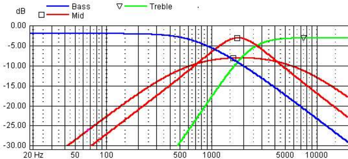
X 1 FD ELECTRIC WITH M40 ( POSITION FLAT-Q3 )
