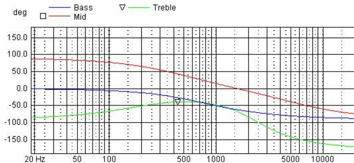
X 1FD PHASE SIMULATION W 600 + M40 + T100
